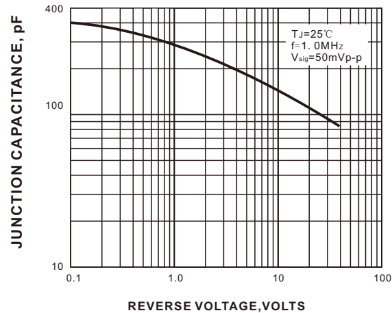
FIG. 5-TYPICAL JUNCTION CAPACITANCE
