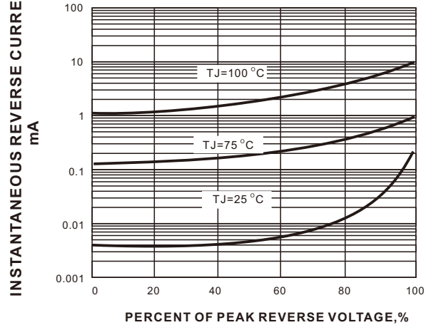
FIG. 4-TYPICAL REVERSE CHARACTERISTICS
