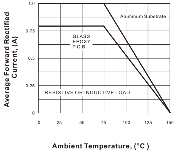
FIG.2 FORWARD DERATING CURVE
